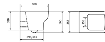
Wall Hung WC
