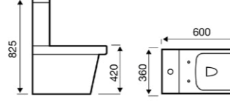
Close to Wall WC
