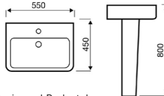
Basin and Pedestal
