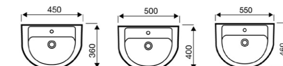
450/500/550mm Basins
