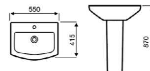
Basin & Pedestal
