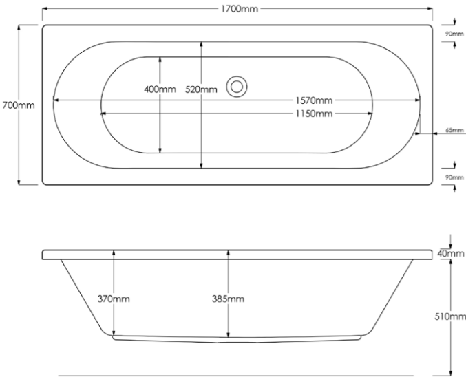
Double-Ended (1700x700mm)
