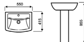
Basin & Pedestal
