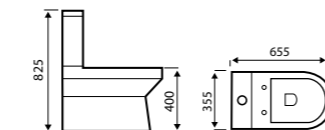
Close-to-Wall WC
