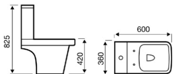
Close Coupled WC
