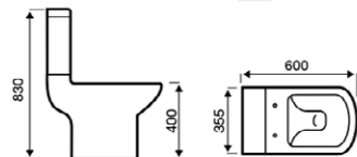
Close Coupled WC
