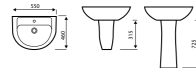
550mm Basin, Semi & Full Pedestal
