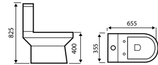
Close Coupled WC
