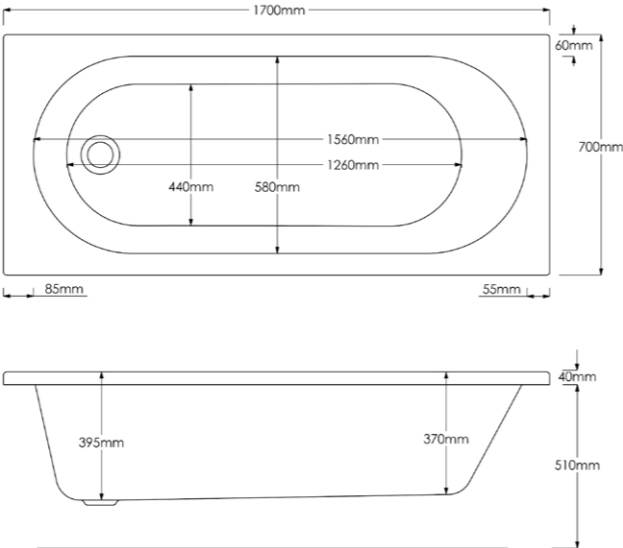
Single-Ended (1700x700mm)
